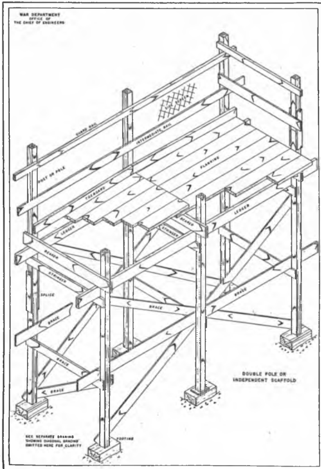
FIGURE 8.—Construction of double pole or independent scaffold.
