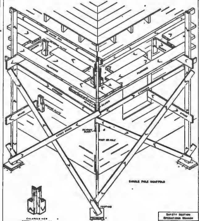
ENLARGED VIEW OF BEAM PLATE
