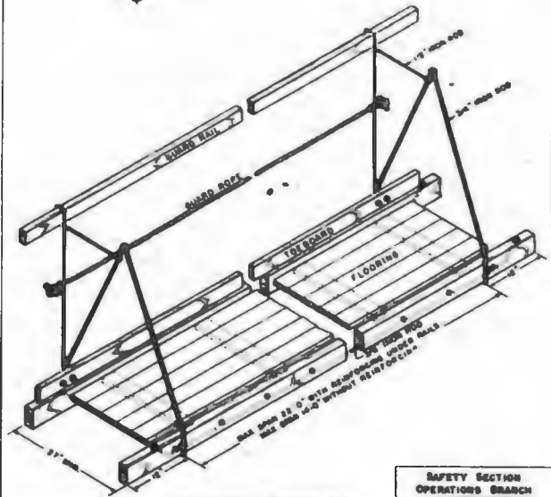
SWINGING SCAFFOLD LADDER PLATFORM TYPE
