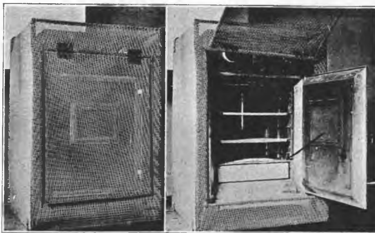
Figure 16. A substantial screen cage placed around a constant-temperature electric oven used to dry samples of explosives. (See paragraph 78.)
