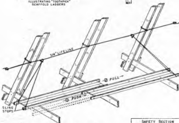
ILLUSTRATING USE OF LIFELINE FOR MOVING SCAFFOLD PLATFORMS
