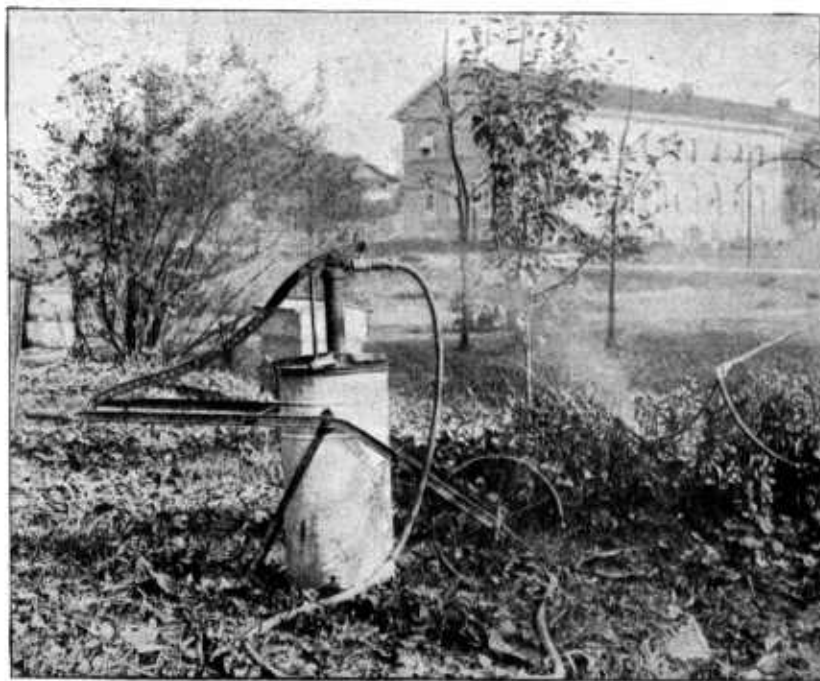
FIG. 13.—Good type of wheelbarrow sprayer effective for small patches. This sprayer holds 12 gallons, and 150 pounds pressure can be kept up when 2 nozzles are used.
